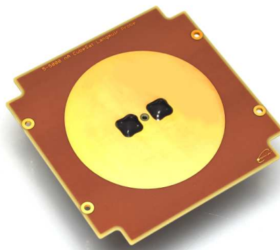
Fig. 5 The piPLASMA/LP Planar Ion Langmuir Probe Panel with Photoelectric Effect Sensor pinhole embedded, Flight Model.
