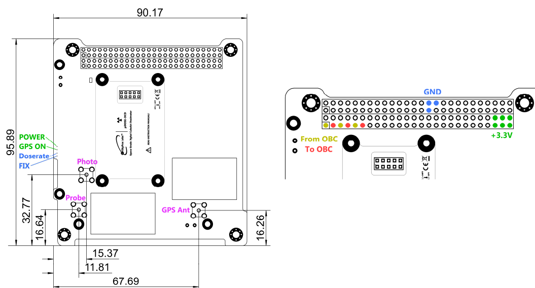
Fig. 2 The piPLASMA Dimensions, Connector locations and device footprint (left), Main PC/104+ Connector Pinout (right), a set of indicating LEDs. NOTE: Dimensions are shown in millimeters.
