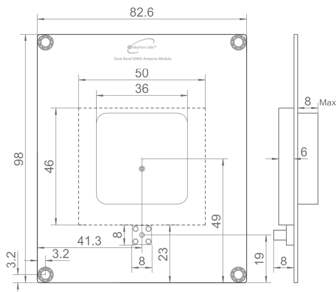
Fig. 2 piPATCH-L1L2 Dimensions drawing in millimeters. Detailed STEP file available for download.
