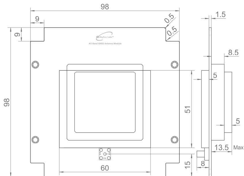
Fig. 2 piPATCH-AllBand-TC Dimensions drawing in millimeters. Detailed STEP file available for download.
