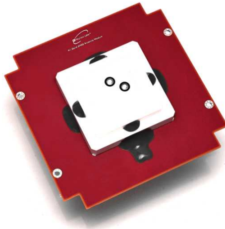
Fig. 3 Engineering Model of the piPATCH-AllBand-TC unit with red Remove Before Flight finish.
