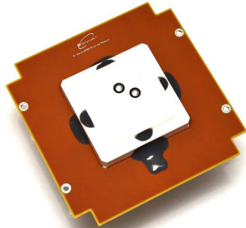
Fig. 1 piPATCH-AllBand-TC/FM Patch Antenna Flight Model.
