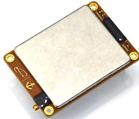
Fig. 1 piAIS/FM, True 2-Channel Dual Band VHF CubeSat AIS Receiver, Flight Model, Top side view.
